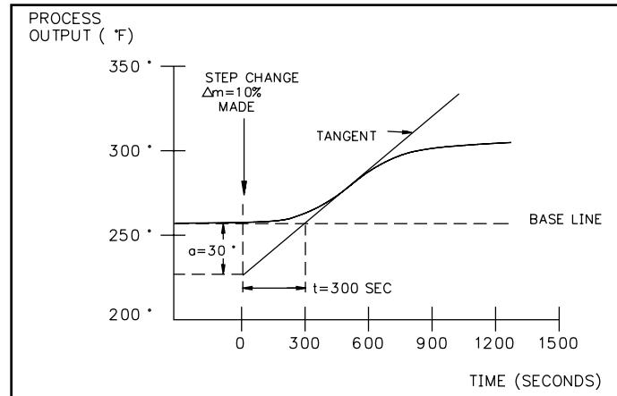
Process Reaction Curve
