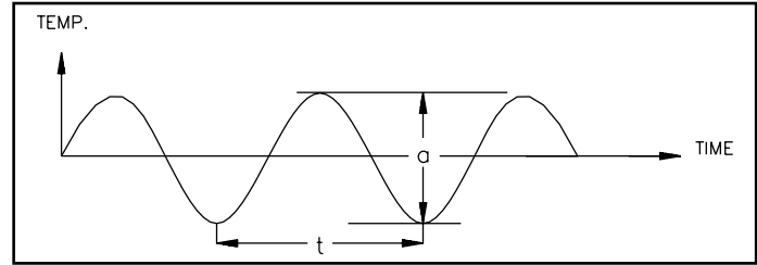
Closed Loop Tuning
