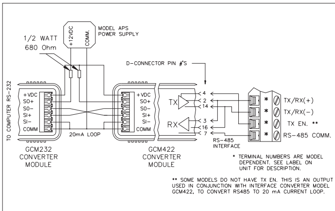
Figure 24, Computer Interface
