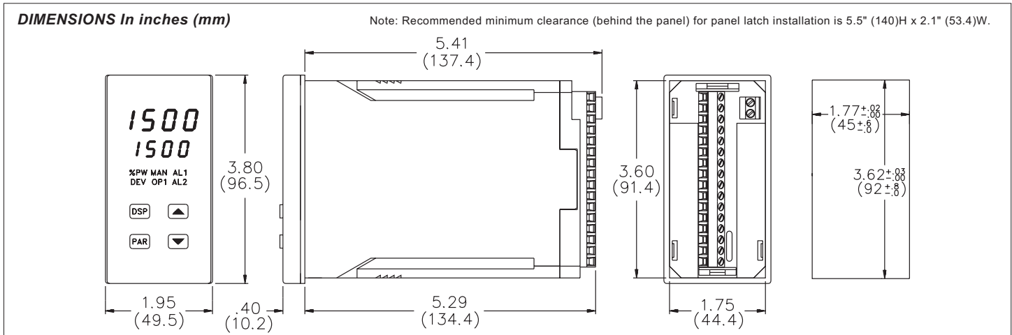
Figure 42, Dimensions
