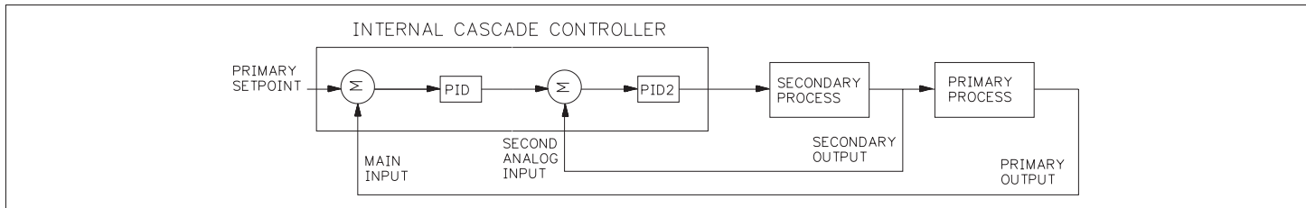
Figure 30, Internal Cascade
