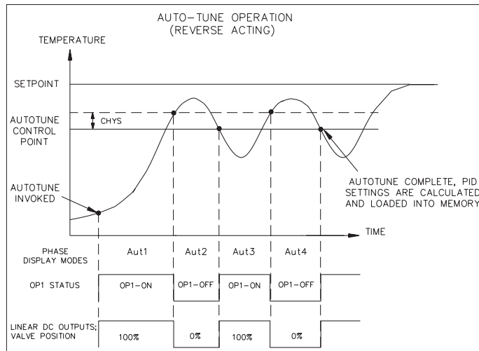
Figure 40, Auto-Tune Operation
