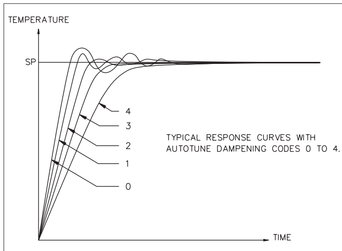
Figure 39, Dampening Code
