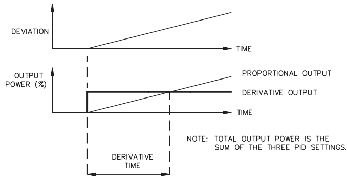
Figure 33, Derivative Time
