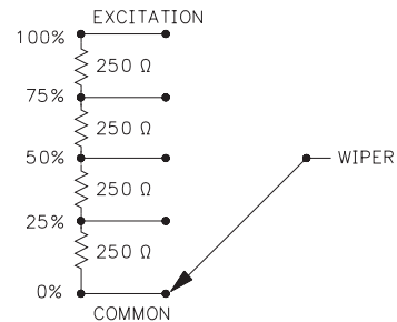
Figure 45, Resistor Divider
