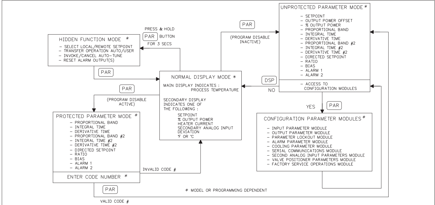
Figure 12, Operational/Programming Modes
