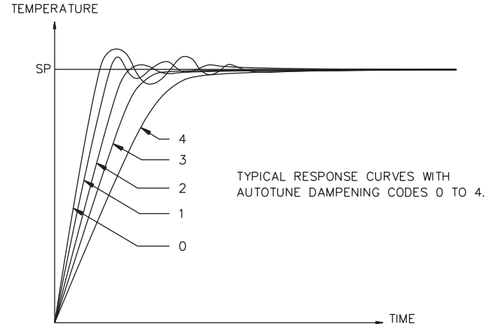
Figure 14, Dampening Code
