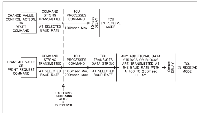
Figure 22, Timing Diagrams
