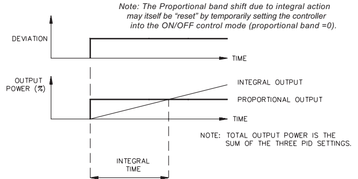
Figure 32, Integral Time
