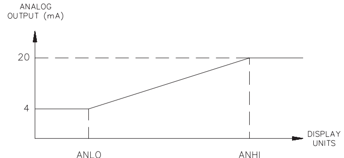
Figure 15, Linear DC Output
