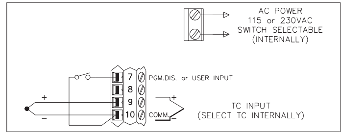
Figure 7, Thermocouple Connection
