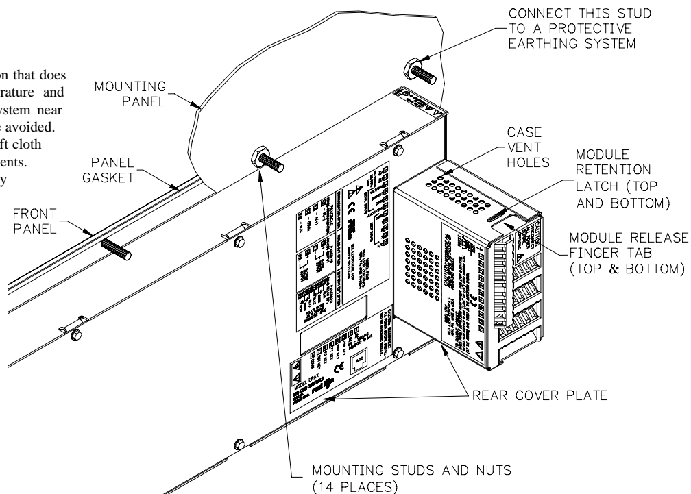
Figure 4, Installing The EPAX Into A Panel
