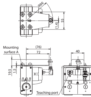
EC-GRB10/GRB13 Individual model number EC-TST-GRB1013 (Individual weight: 0.06kg / Material: Stainless steel)
