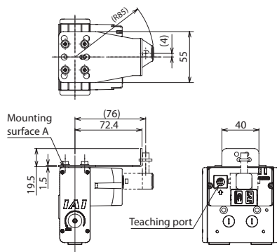
EC-GRB8 Individual model number EC-TST-GRB8 (Individual weight: 0.06kg / Material: Stainless steel)
